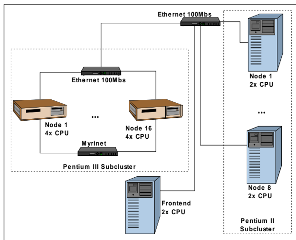
Figure 1. The Gescher Cluster Architecture
