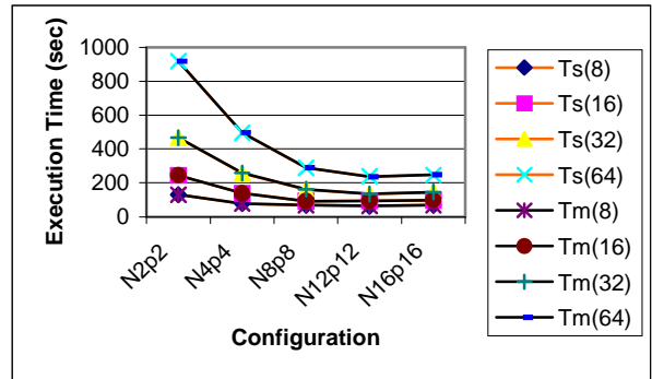
Figure 5. Simulation and Measurement Results on Monoprocessor Nodes
