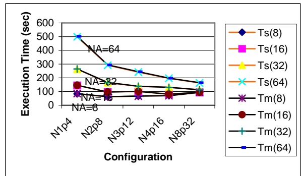
Figure 6. Simulation and Measurement Results on SMP Nodes
